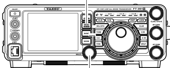
Manopola MULTI
