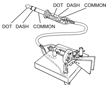
Manipolator
